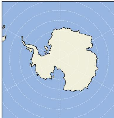
MRB: years 1990 to 2017 n=23118
