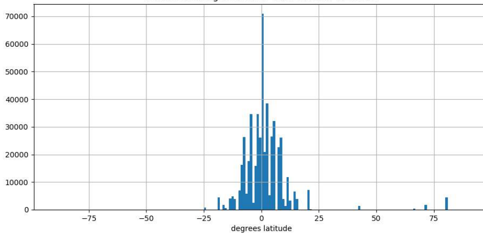
MRB: # vs 1-degree lat bin. 1990 to 2017 n=23118
